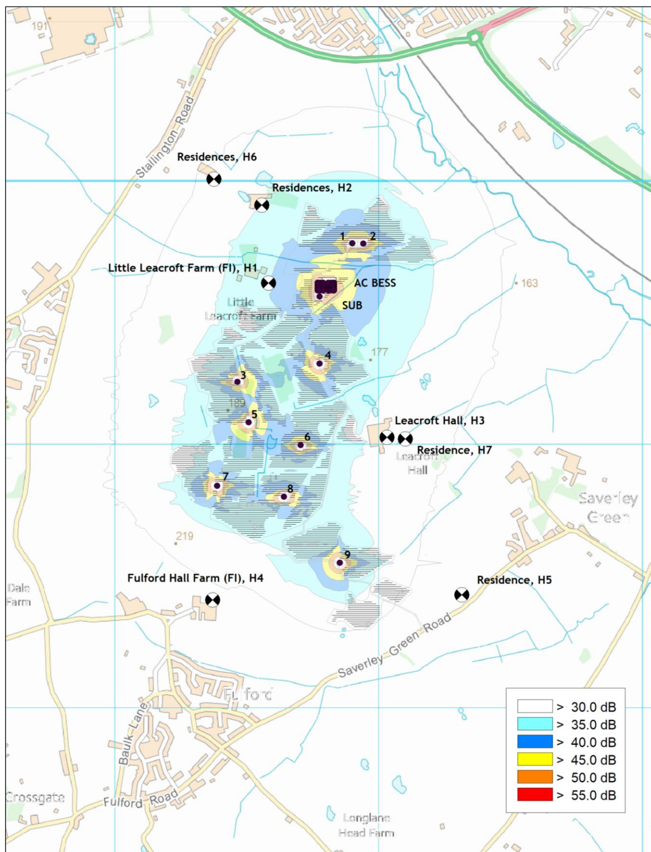
Figure 1 - Noise Contour Plot, dB L Ar
